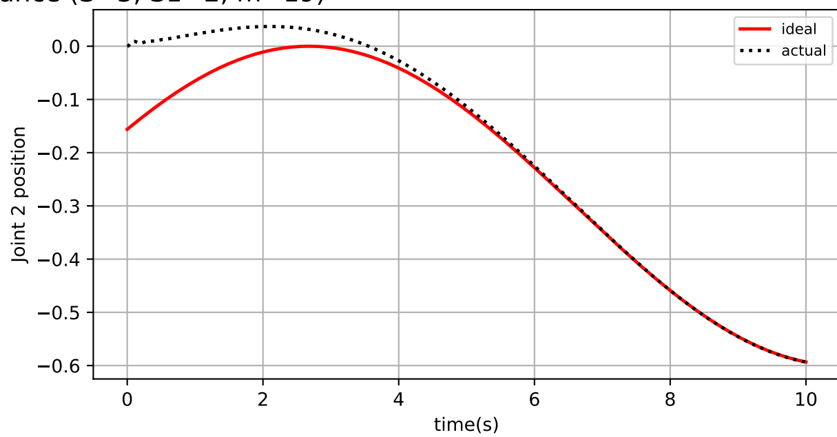
Position Tracking Performance (S=3, S1=2, m=19)
